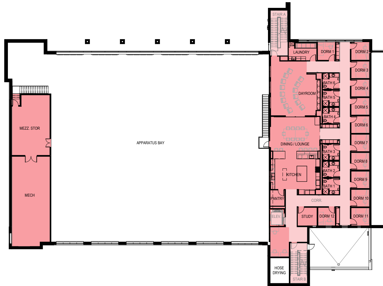
SECOND FLOOR AREA PLAN Scale: 1" = 30'-0"
